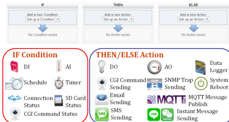
▲ The function overview of IF-THEN-ELSE rule engine
